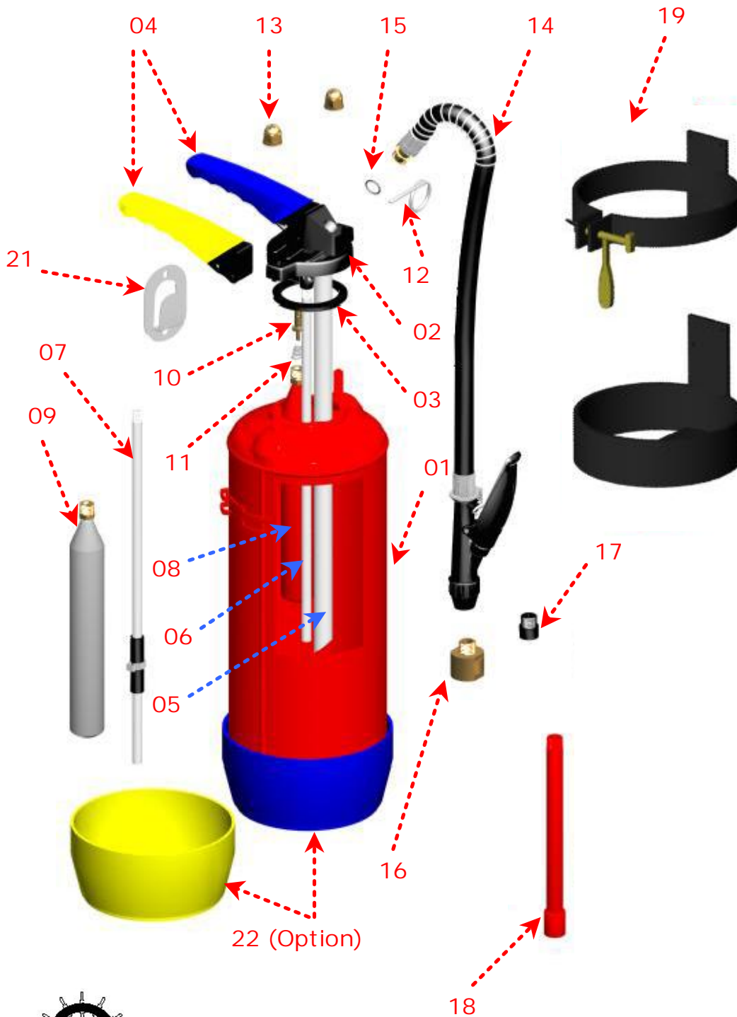
Vulcain Poudre Powder Extinguisher
